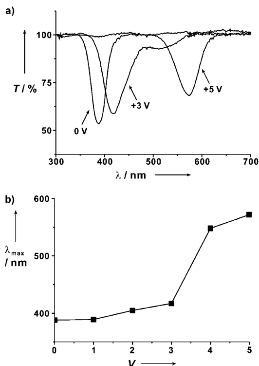
Figure 2. Optical responses of a PS- b -P2VP photonic pixel filled with LiCl electrolyte in response to the applied voltage (0–+5 V): a) UV/Vis transmission spectra and b) variation in \lambda_{\text{max}} with bias voltages.
